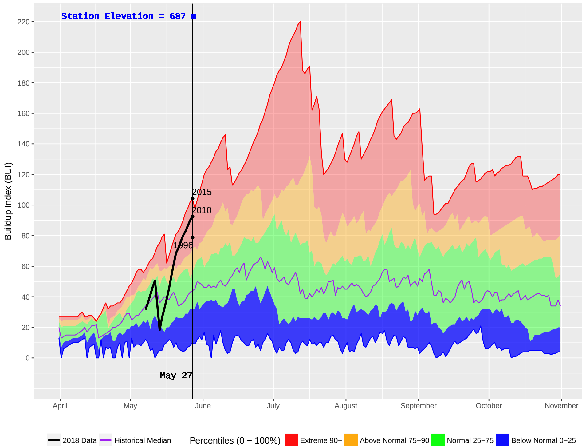
KETCHIKA (444) : Historical (1986–2016) and Current (2018) Noon Buildup Index (BUI)
