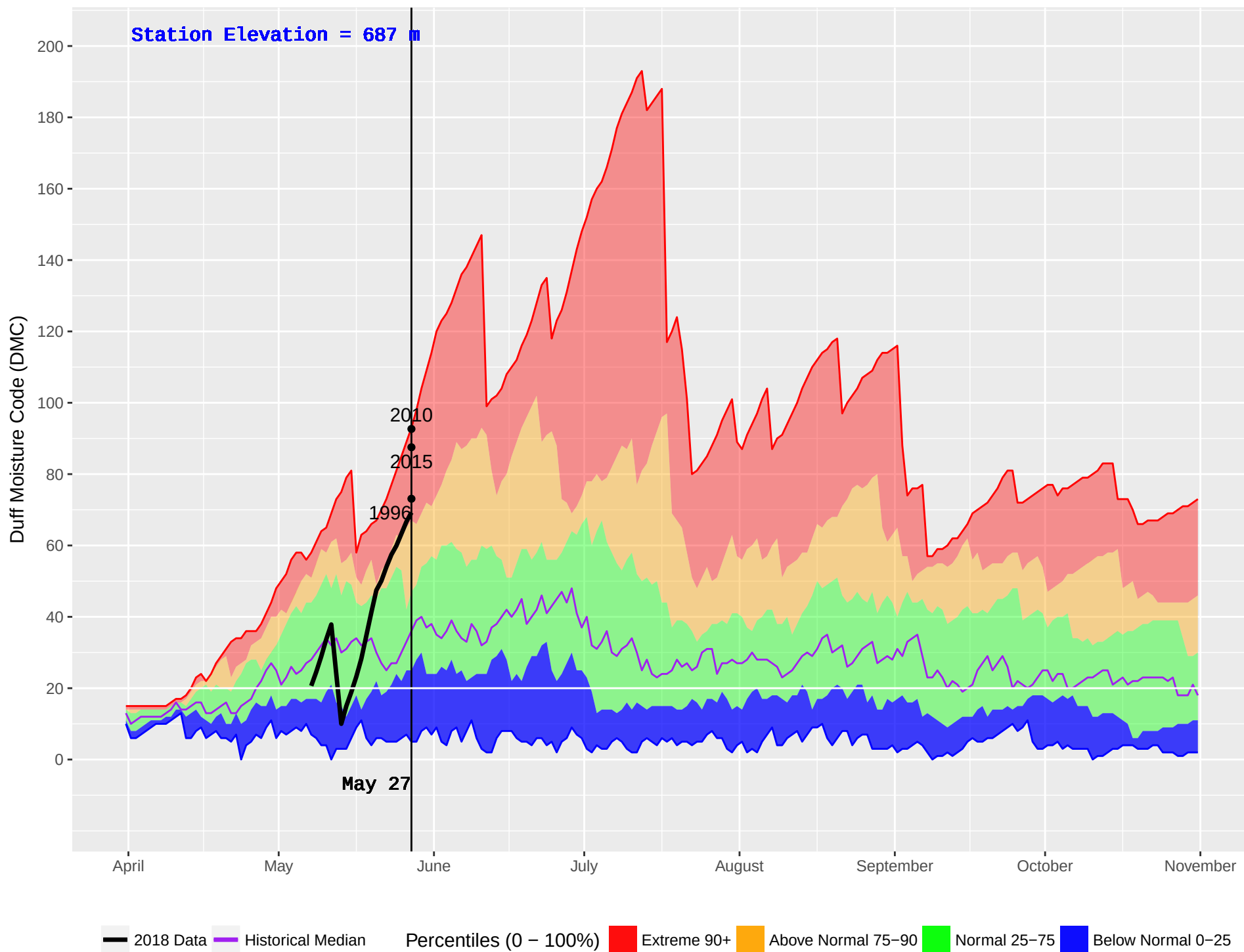
KETCHIKA (444) : Historical (1986–2016) and Current (2018) Noon Duff Moisture Code (DMC)
